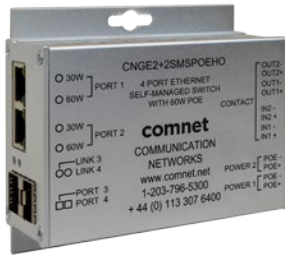
CNGE2+2SMS and CNGE2+2SMSPOE[HO] 4-Port All-Gigabit Self-Managed Switches with 30 W PoE+ / 60 W Universal PoE
